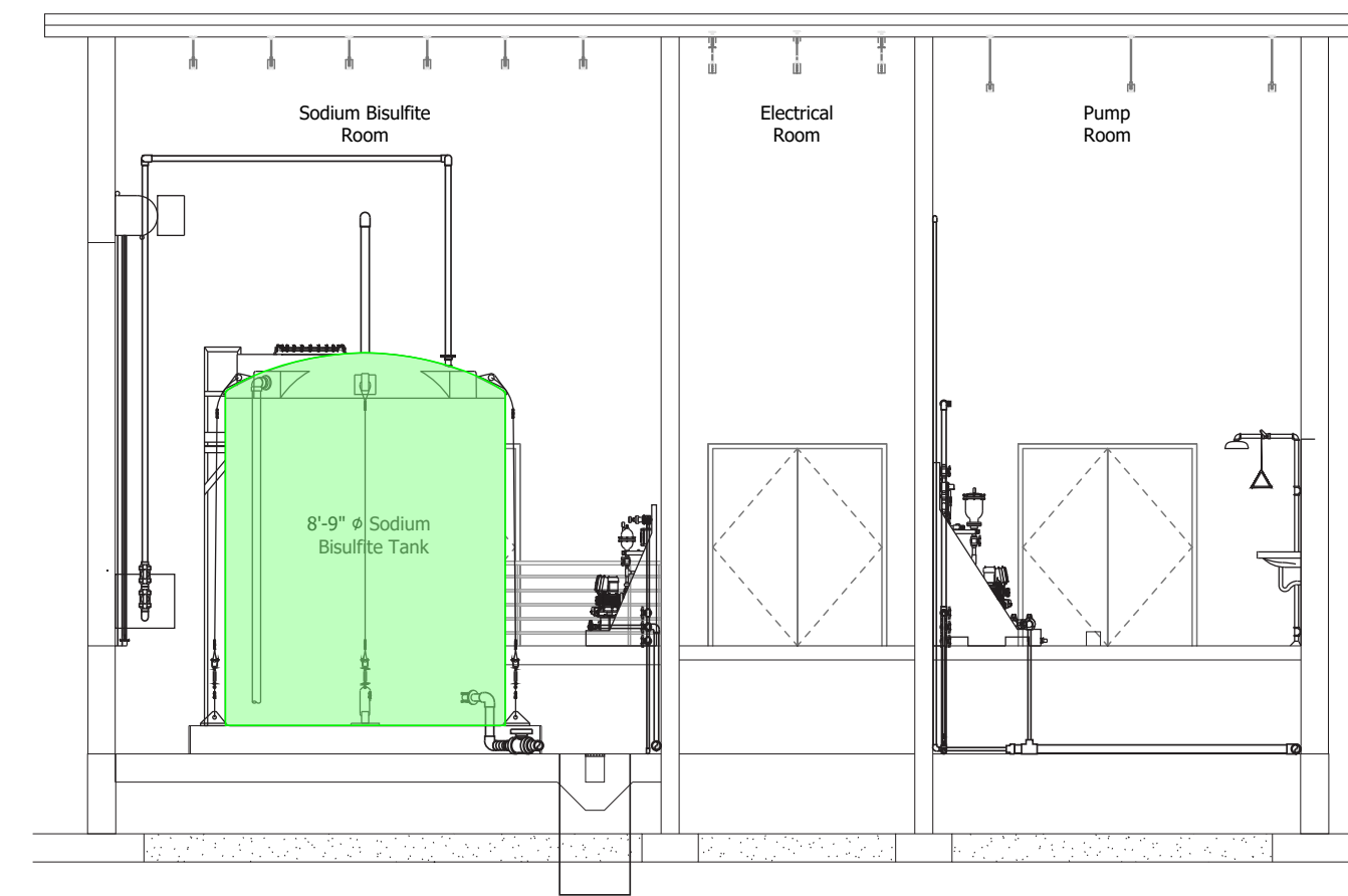
Section View
