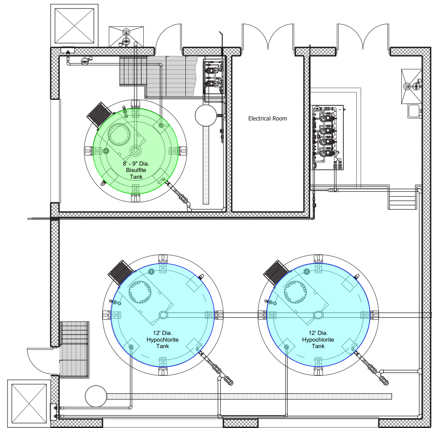
Plan View
